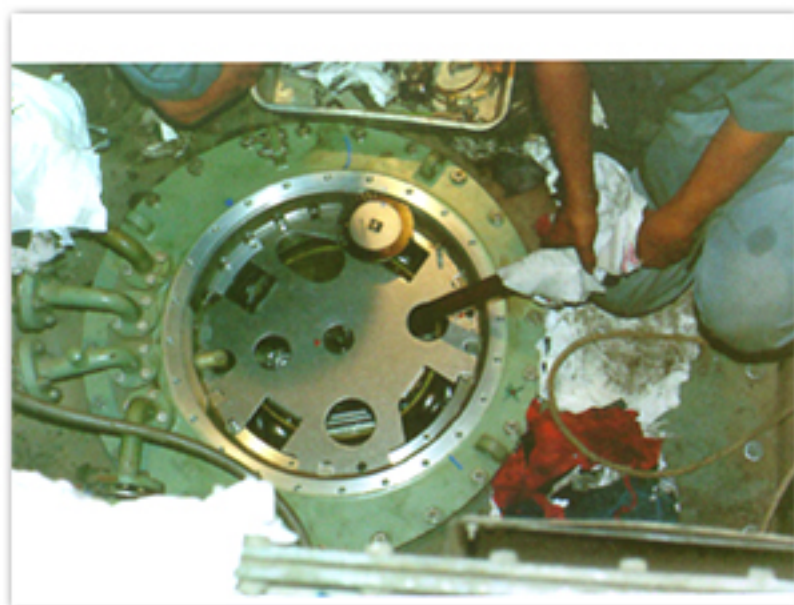
"MR" on Load Tap Changer Inspection, Oil Replacing and Overhauling
