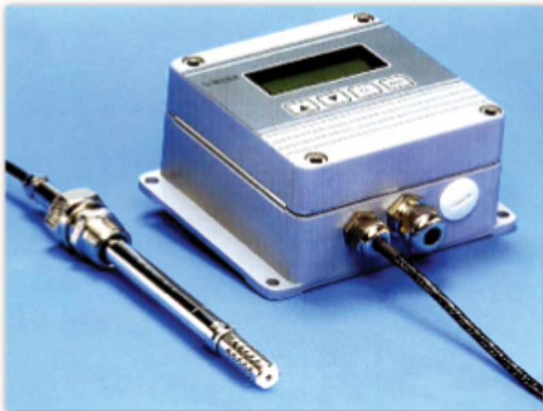
"Vaisala-Finland" HMP 228 Moisture and Temperature Transmitter For Oil
